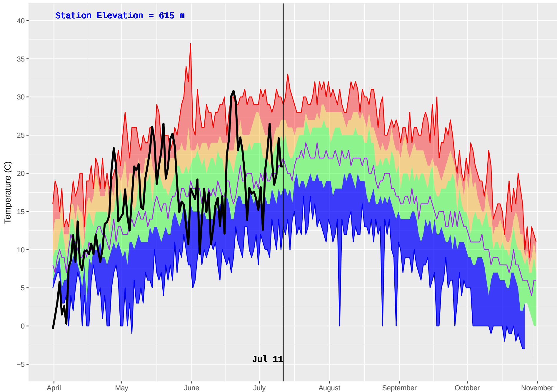
HIXON (187) : Historical (1976–2016) and Current (2018) Noon Temperature
