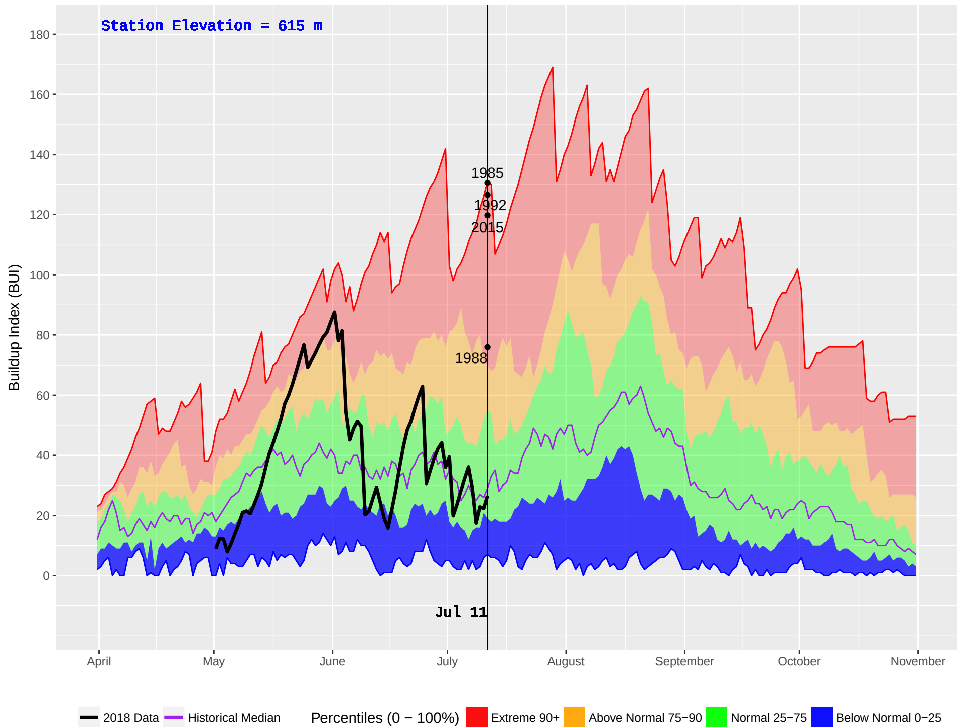
HIXON (187) : Historical (1976–2016) and Current (2018) Noon Buildup Index (BUI)
