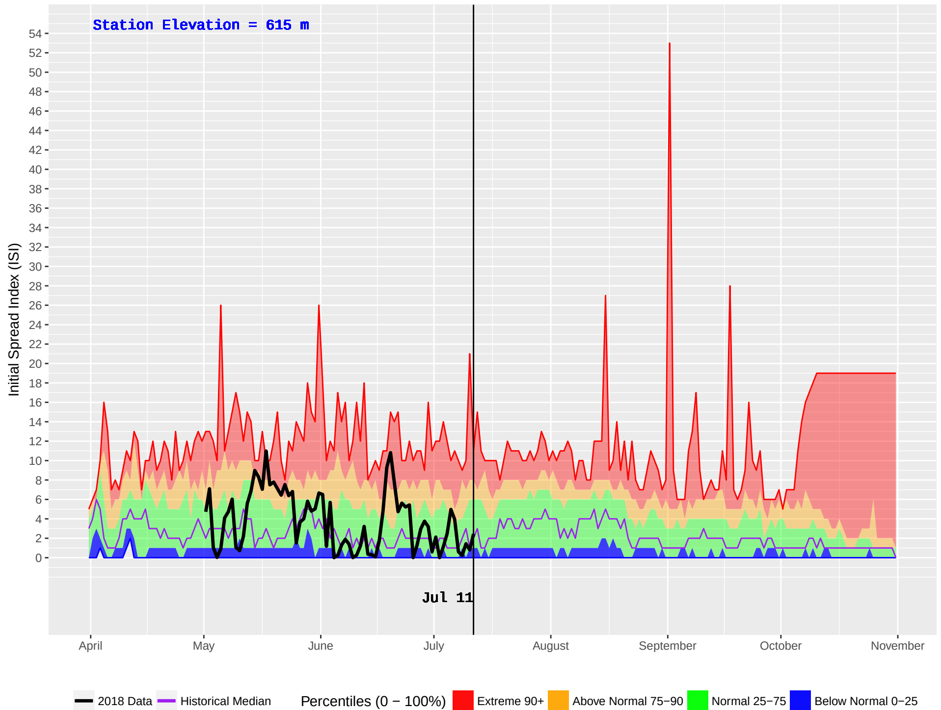
HIXON (187) : Historical (1976–2016) and Current (2018) Noon Initial Spread Index (ISI)
